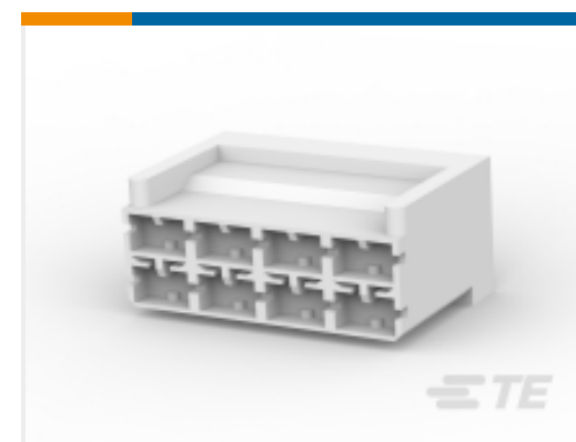
TE Part # 926646-3 PL 250 8P HOUSING PA6.6 ZYTEL 101NATURAL
